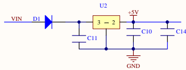
Power Regulator
