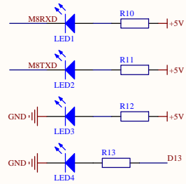
Indicator Unit
